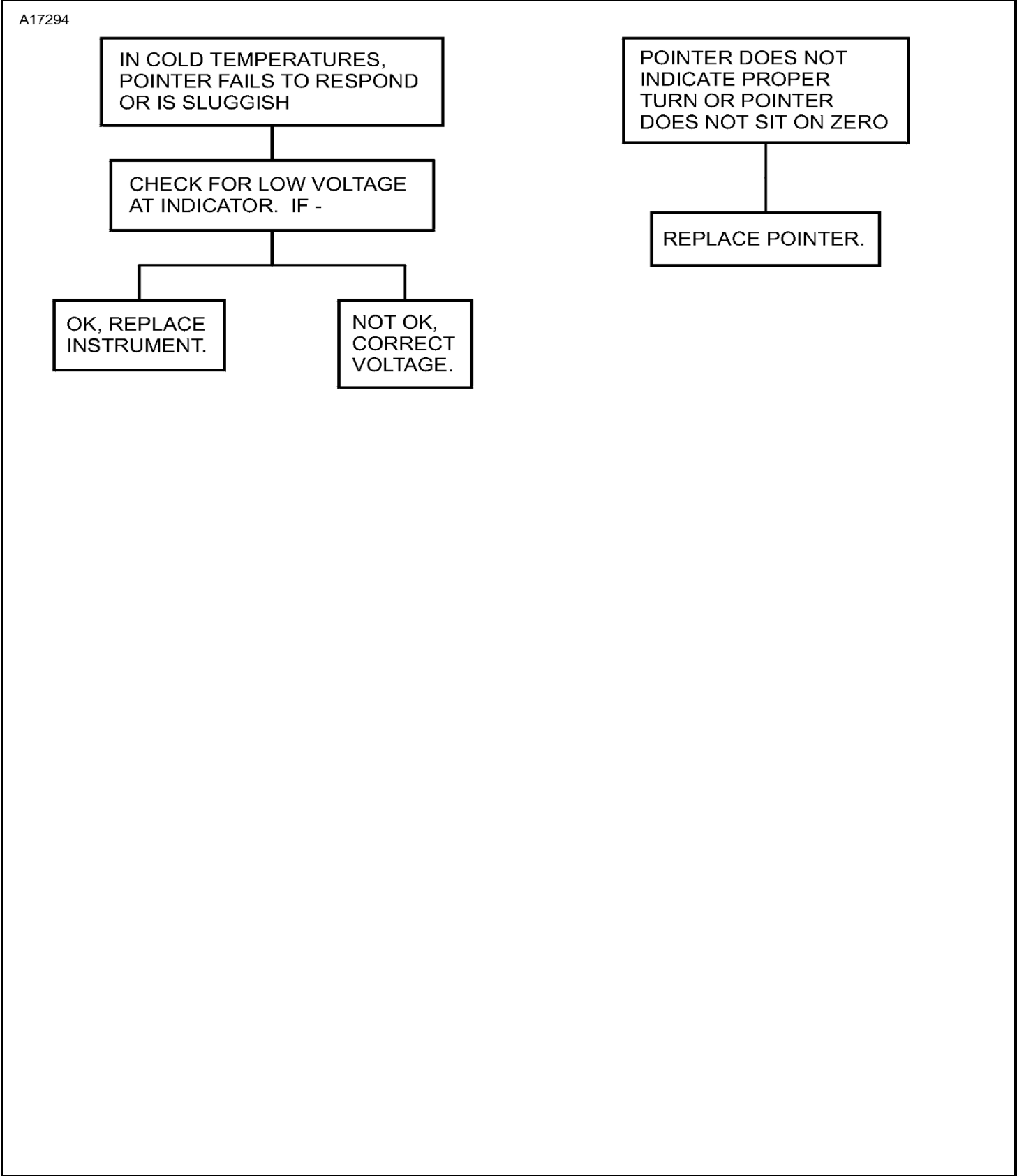
Figure 101 : Sheet 3 : Turn and Bank Indicator Troubleshooting Chart
